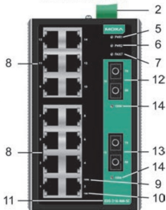
EDS-316-MM-SC Front Panel View
