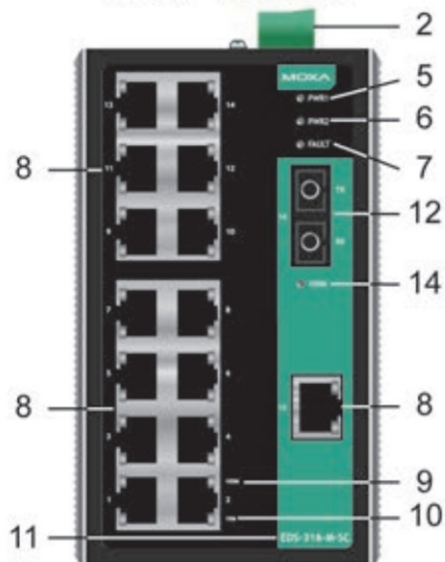
EDS-316-M-SC Front Panel View
