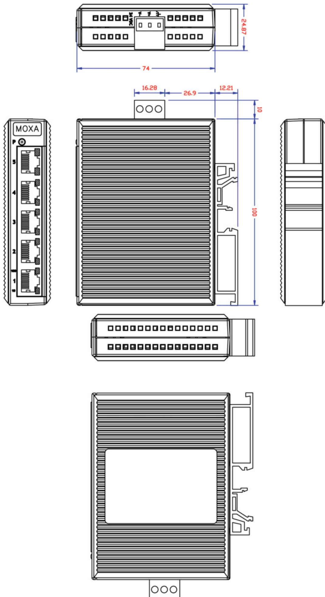
DIN-Rail Mounting
