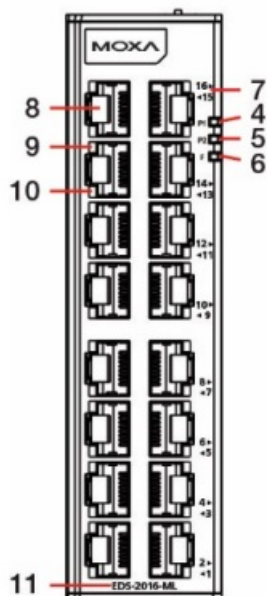
Front Panel View
