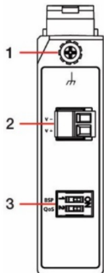
Top Panel View
