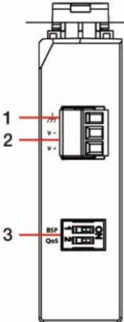
Top Panel View
