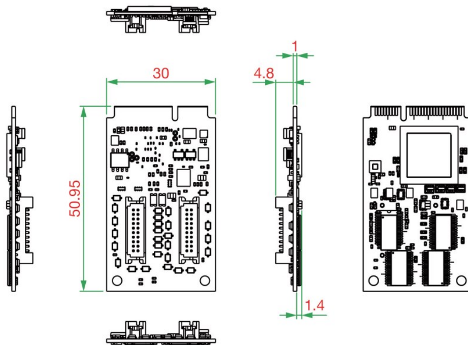
Mainboard Dimensions (Mini PCIe)
