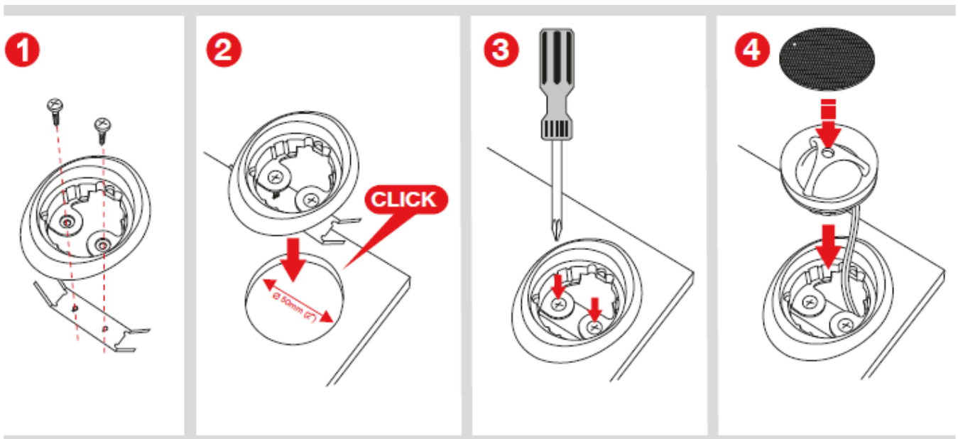
Option 2: Surface mounting
