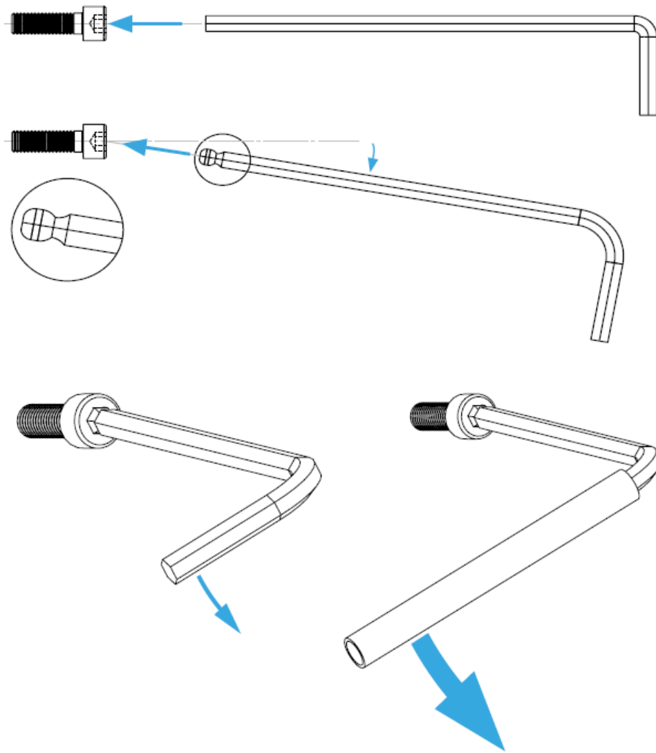
UNIVERSAL CONNECTOR
