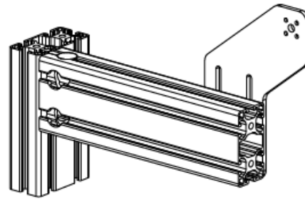
Alternative mounting to get the collective closer to the seat.
