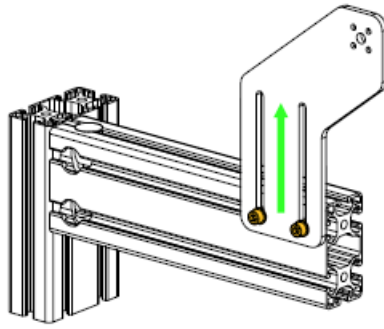
Alternative mounting allows for higher collective positions.
