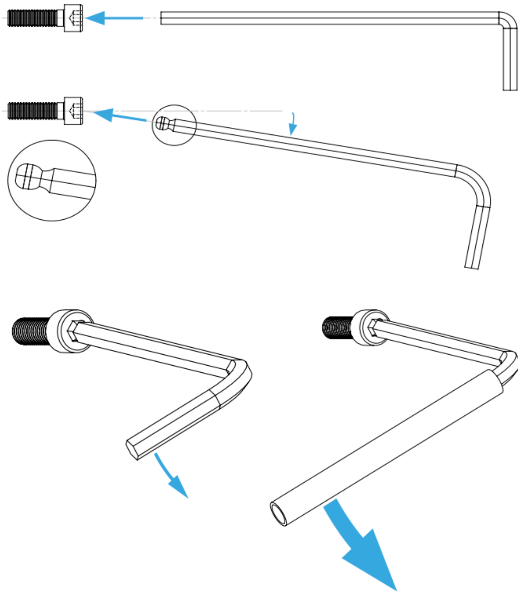
UNIVERSAL CONNECTOR
