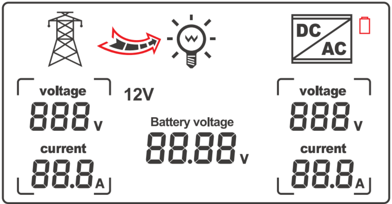
Automatic mode switching inverter state
