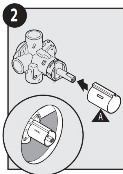
Slide Stop Tube (A) onto valve.
