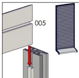
SLOTWALL EXTRUSION
