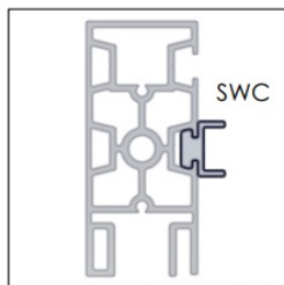
SLOTWALL CHANNEL
