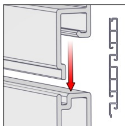
SLOTWALL EXTRUSION
