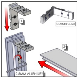
CORNER CLEAT
