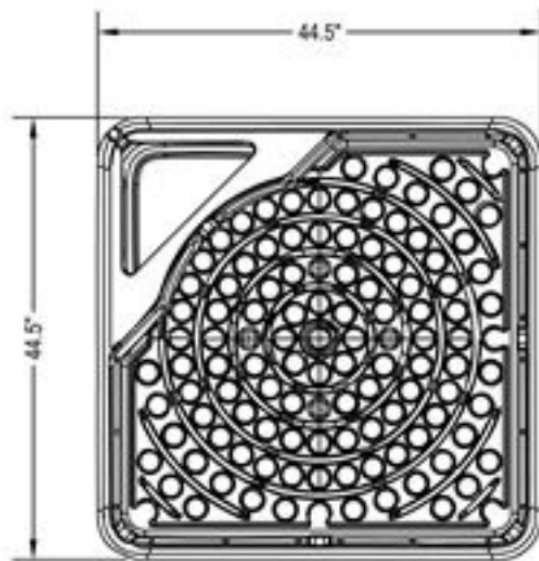
PLAN VIEW AQUABASIN LARGE MODEL: #98134 WEIGHT: 46.5 LBS
