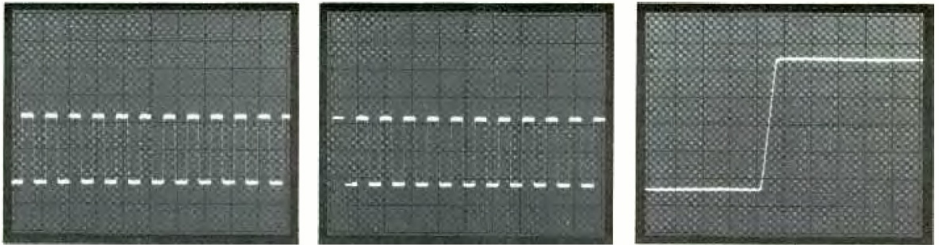
Fig. 10. Delayed sweep adds precise amount of time between trigger point (left) and beginning of sweep (center). By adjusting controls to display one transition of input waveform (right), you can obtain risetime measurement modes, labeled on the front panel NO DLY, INTENS and DLY'D.
