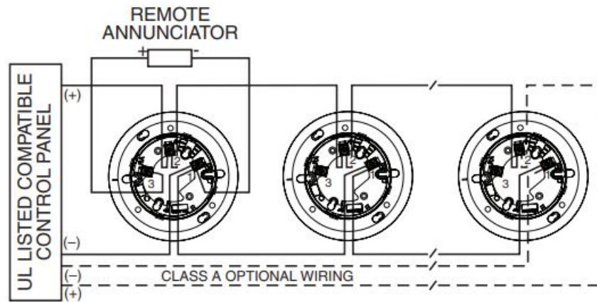
FIGURE 1. WIRING DIAGRAM
