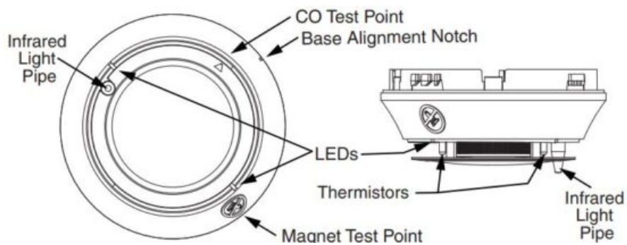
FIGURE 4. CLEANING THE FIRE/CO DETECTOR
