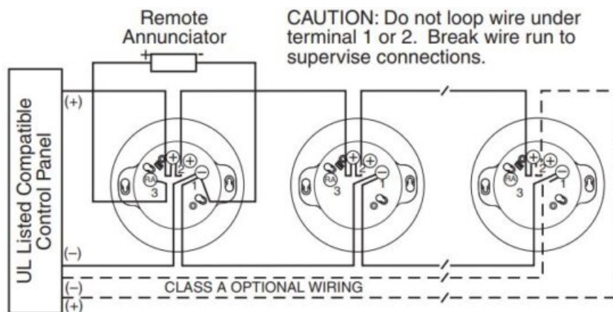
FIGURE 2. WIRING DIAGRAM
