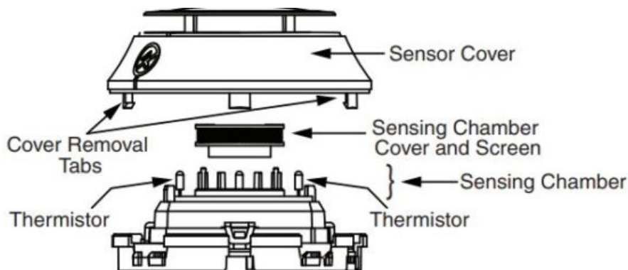
FIGURE 4. CLEANING THE PHOTO/HEAT DETECTOR
