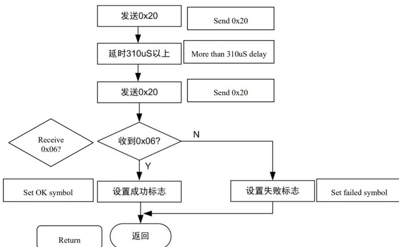
Figure 2.2 Determination of communication baud rate
