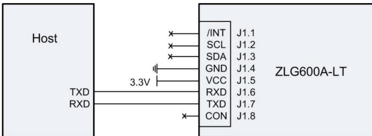
Figure 2.1 UART typical application in auto detection mode
