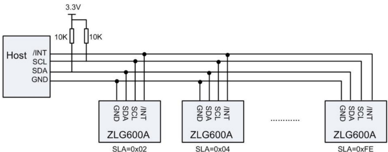
Figure 2.4 I 2 C multi-slave connection diagram
