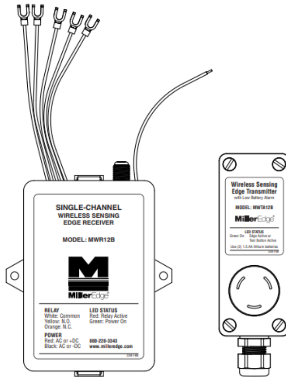
IMAGE 2: MWRTA12B (MWR12B + MWTA12B) Single-Channel Wireless Edge System with Low Battery Alarm
