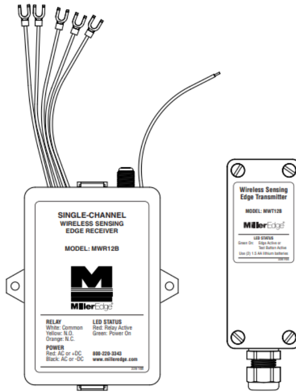
IMAGE 1: MWRT12B (MWR12B + MWT12B) Single-Channel Wireless Edge System
