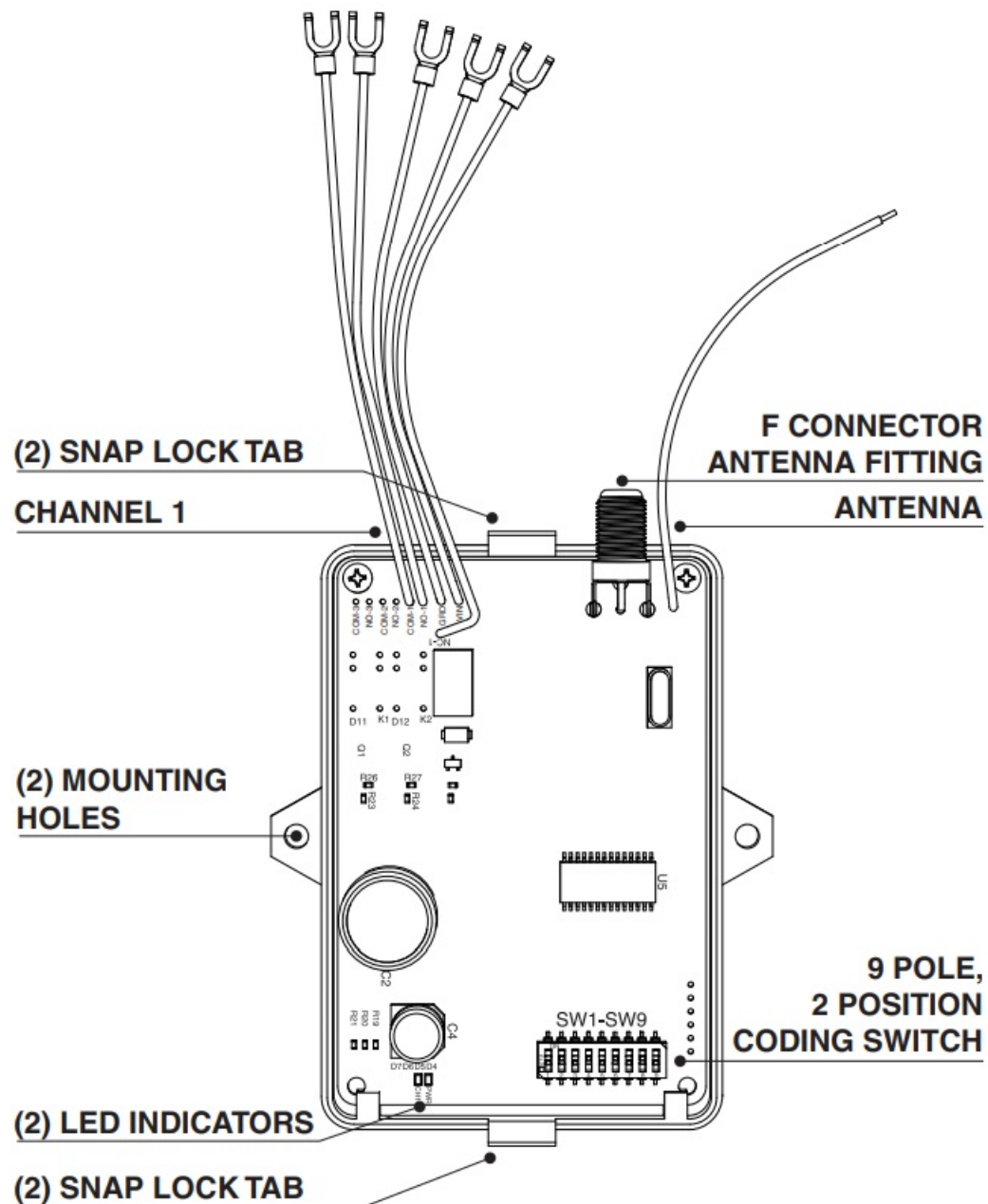
IMAGE 3: RECEIVER BASE DETAIL
