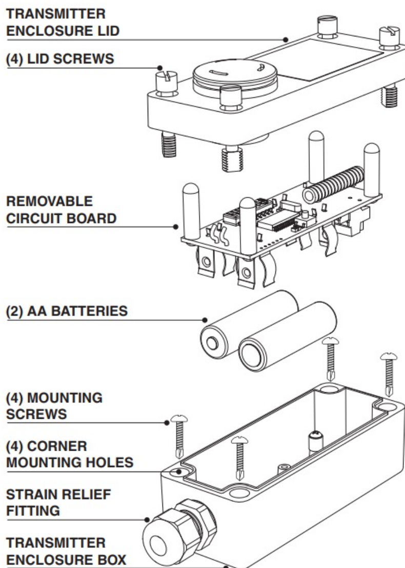
IMAGE 4: TRANSMITTER ASSEMBLY
