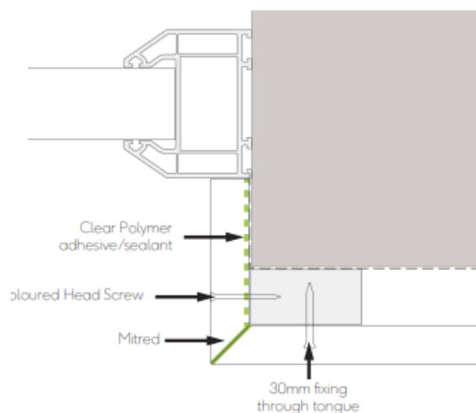
Fig. 13 - Window/door jamb with mitred joint
