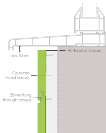
Fig. 3 - Window/door sill detail
