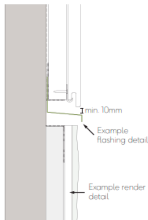
Fig 23 - Installing cladding above render
