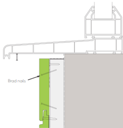
Fig. 16 - Window/door sill junction detail - brad nails
