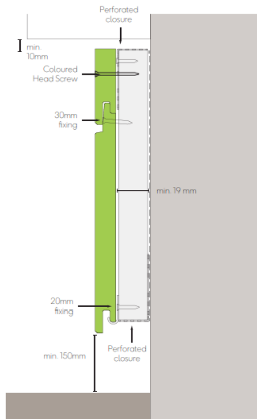
Fig.1 - Top & bottom of cladding detail
