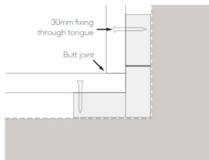
Fig. 9 - Internal butt jointed detail
