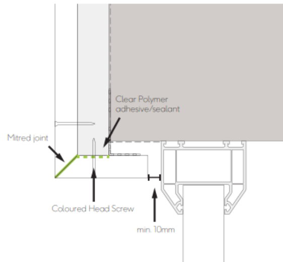
Fig. 14 - Window/door head with mitred joint
