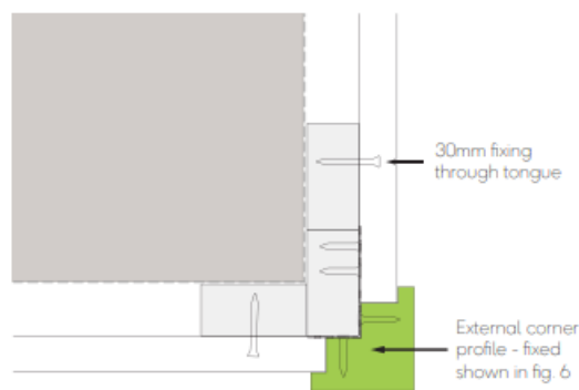
Fig. 8 - External corner detail
