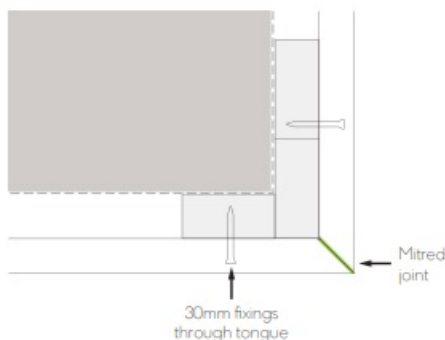
Fig. 10 - External mitred corner detail
