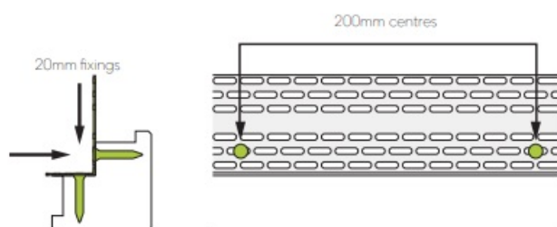
Fig. 6 - Use of perforated closure on corner profiles
