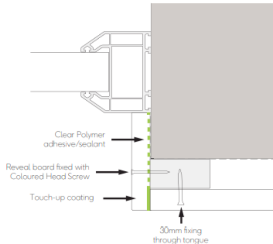
Fig. 11 - Window/door jamb with fascias
