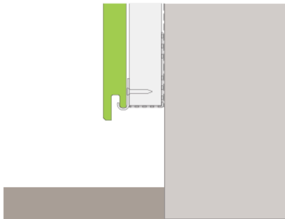
Fig. 19 - First board install
