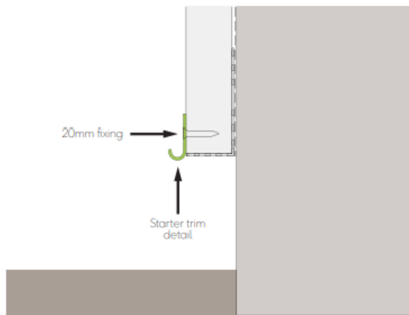
Fig. 18b - Starter trim detail
