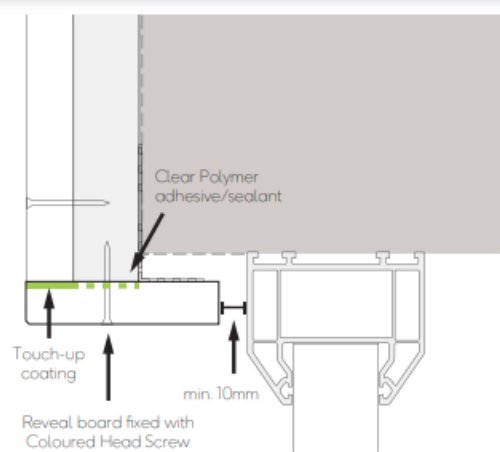
Fig. 12 - Window/door head with Reveal board
