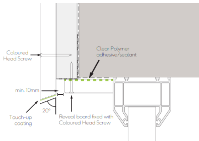
Fig. 15 - Window/door head with angled cut
