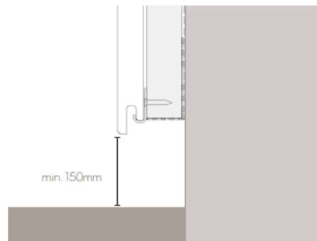
Fig. 4 - Install detail above ground level
