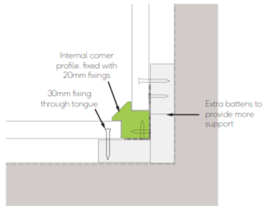
Fig. 7 - Internal corner detail
