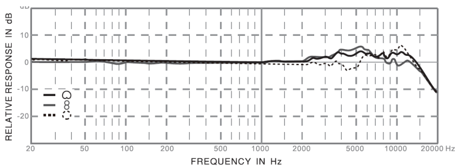
MK300 Typical Frequency Response
