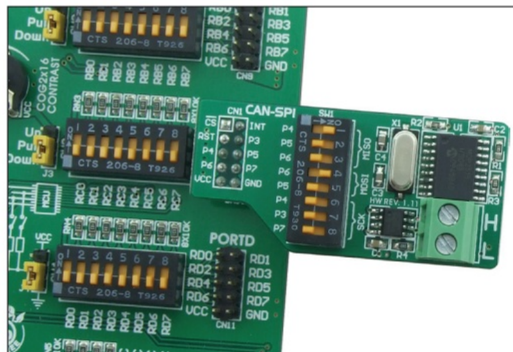
Figure 2: CAN-SPI board connected to a development system
