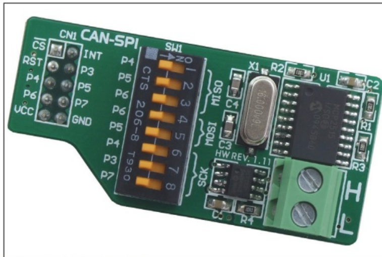
Figure 1: CAN-SPI additional board
