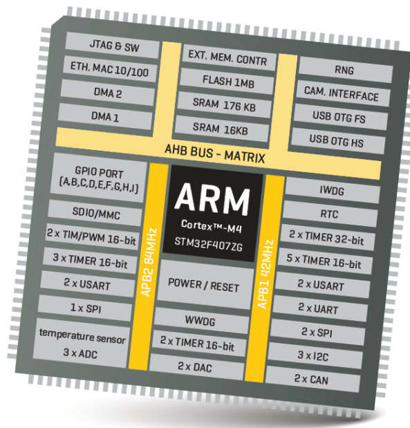
Figure 1: STM32F407ZGT6 MCU block schematic
