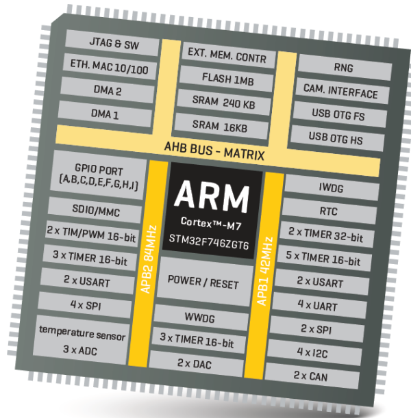
Figure 2: STM32F746ZGT6 MCU block schematic
