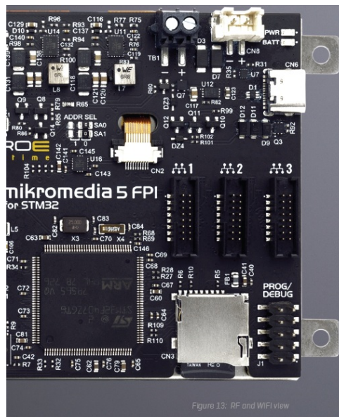
Figure 13: RF and WiFi view
