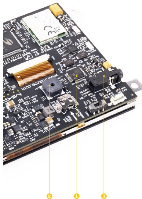
Figure 15: mikromedia 5 FPI back view
