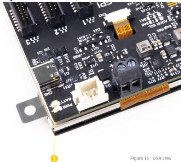
Figure 12: USB view
