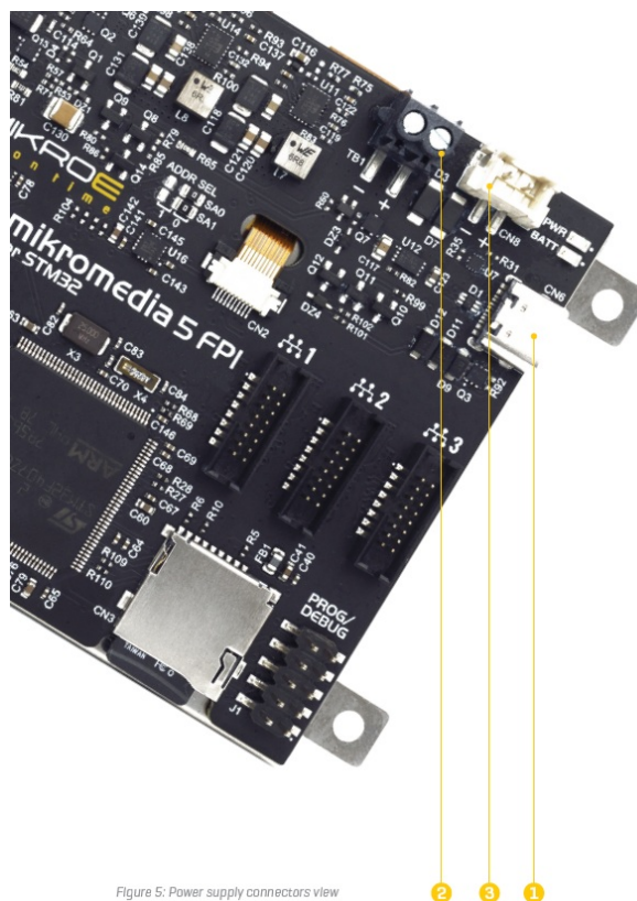
Figure 5: Power supply connectors view
