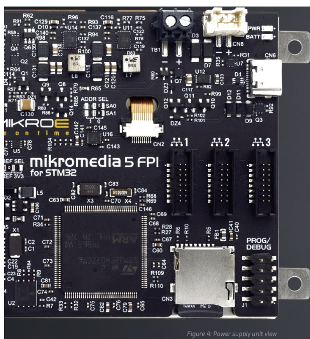
Figure 4: Power supply unit view
