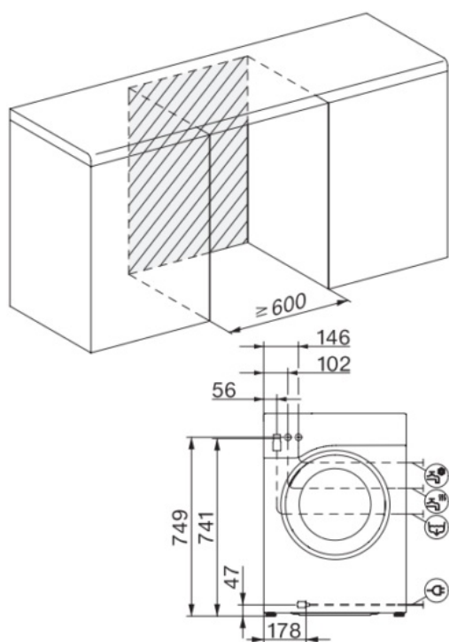
W1 drawing, facia 5 degree, measures in mm
