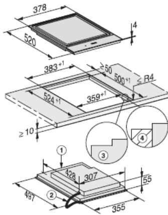
CS7632FL, flush (installation drawing)
