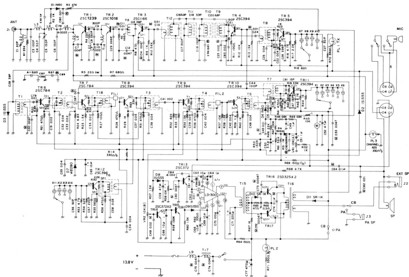
WIRING DIAGRAM
