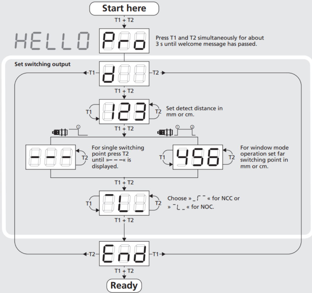
Diagram 1: Set sensor parameters numerically using LED display
