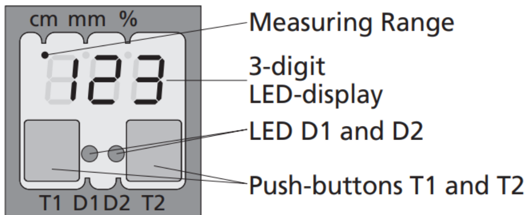
Fig. 3: TouchControl/LED display
