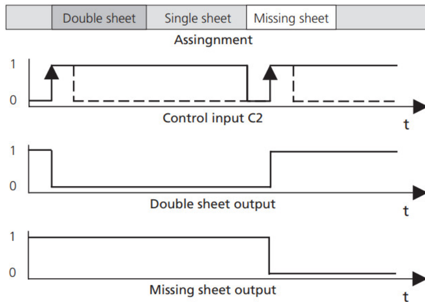
Fig. 8: Trigger mode edge-controlled
