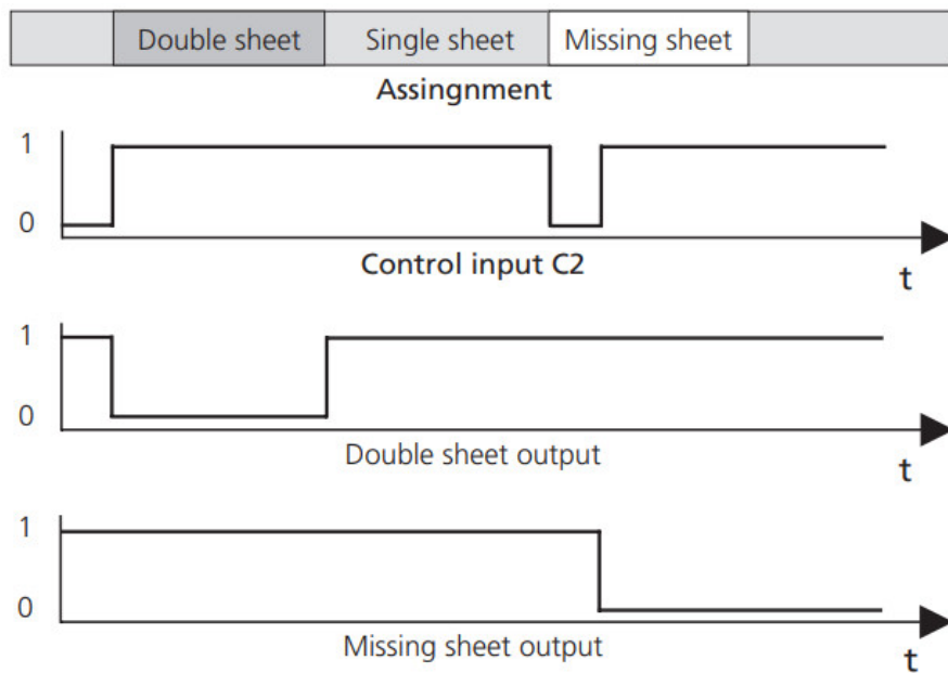
Fig. 9: Trigger mode level-controlled
