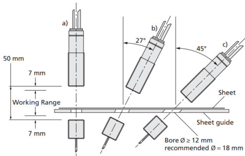
Fig. 3: Mounting and installation positions
