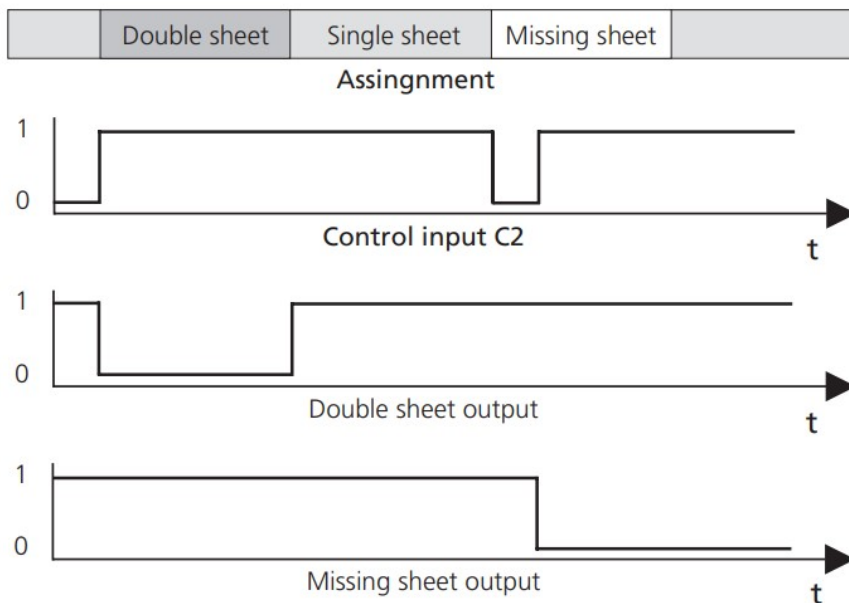
Fig. 9: Trigger mode level-controlled
