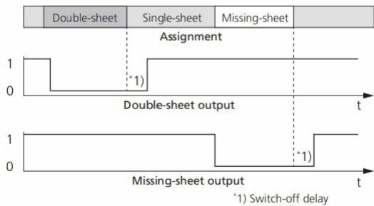
Fig. 6: dbk-4/CD/O/QP (double-sheet output only) dbk-4/CDD/O/QP and dbk-4/CEE/IS/QP, Free Run Mode
