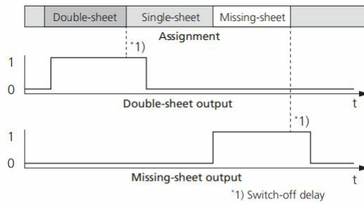
Fig. 7: dbk-4/CDD/O/QP/POD, Free-Run-Mode
