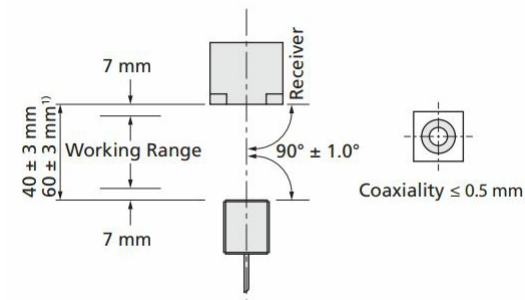
Fig. 2: Installation and working range 1) optional with dbk-4/CDD/O/QP E+S/POD
