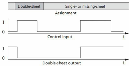
Fig. 5: dbk-4/CD/O/QP, Trigger-Mode
