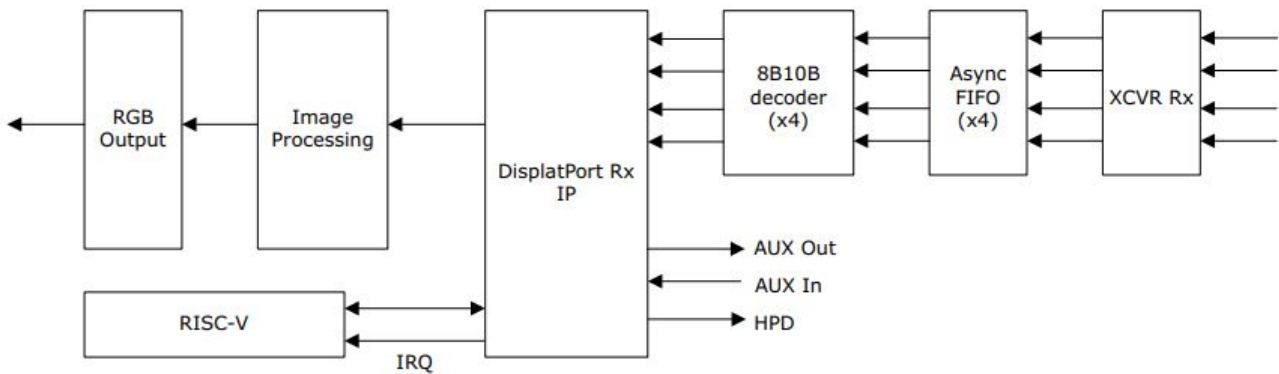
Figure 4 • Typical application for DisplayPort Rx IP
