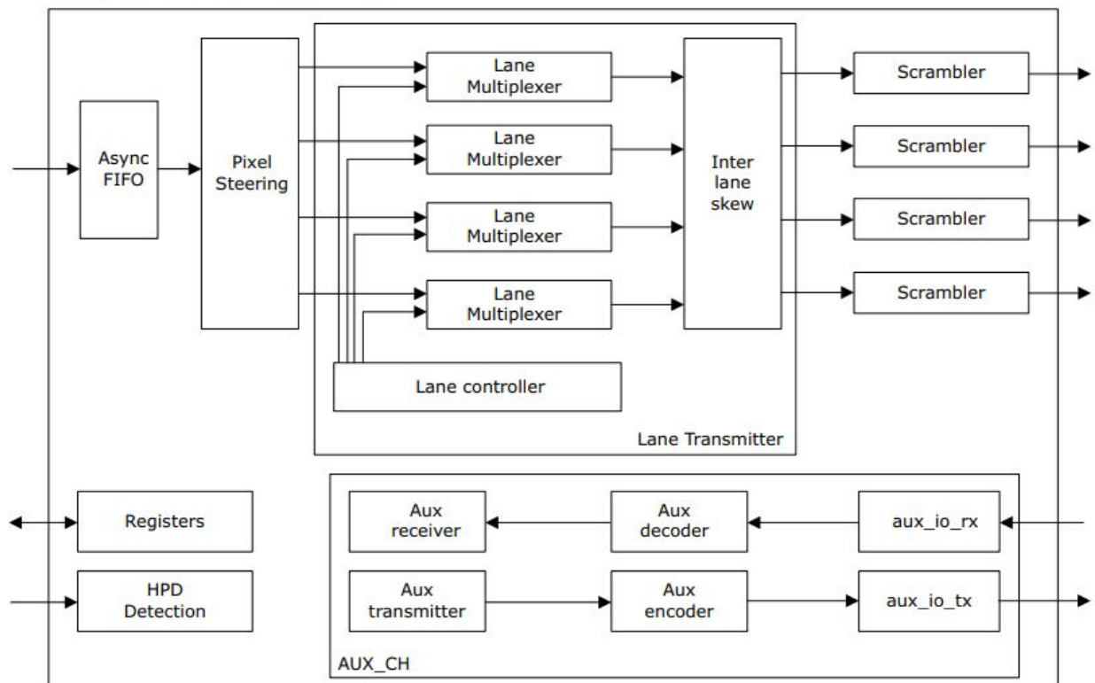
Figure 1 • DisplayPort Tx IP Implementation
