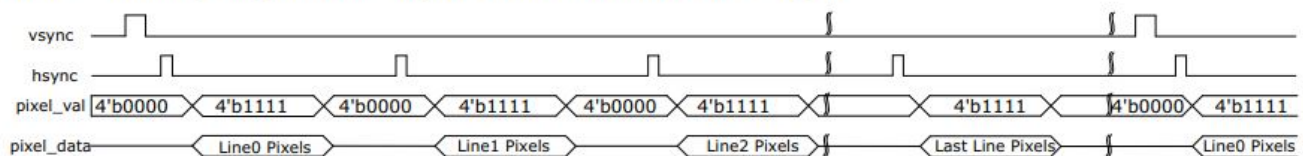
Figure 6 • Timing Diagram for Output Video Stream Interface Signal
