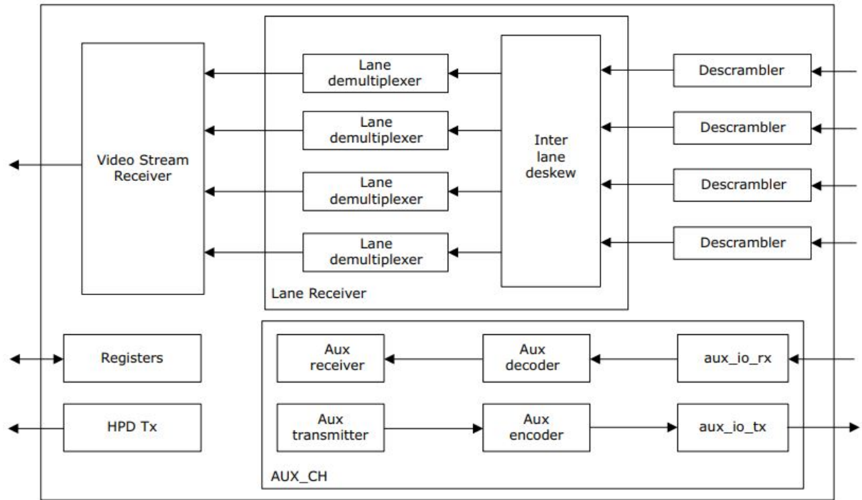
Figure 2 • DisplayPort Rx IP Implementation
