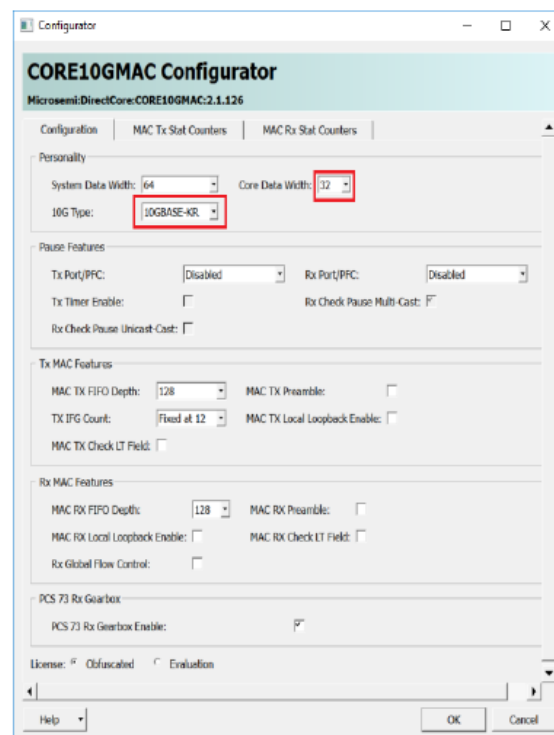
Figure 5 • Core10GMAC Configuration for 10GBASE-KR Designs
