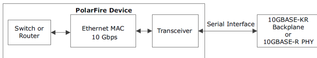
Figure 1 • Sample Ethernet Application
