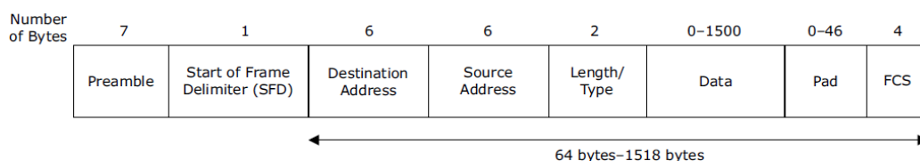
Figure 13 • Standard Ethernet Frame Format
