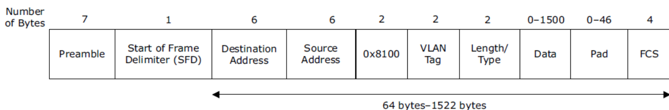
Figure 14 • Ethernet VLAN Frame Format
