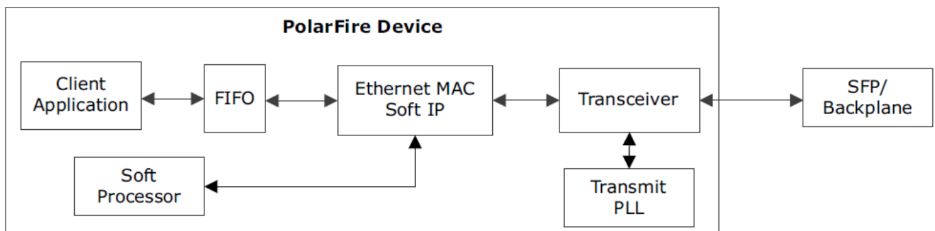
Figure 3 • Sample Ethernet Application Using Microsemi IP Cores
