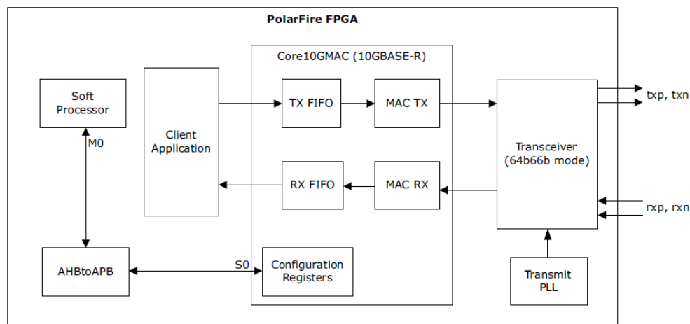
Figure 11 • 10GBASE-R System Diagram
