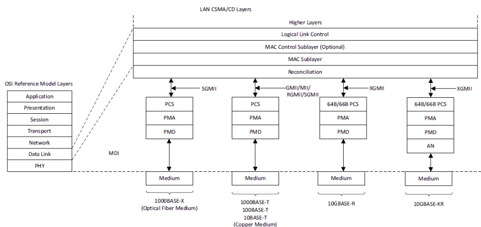
Figure 10 • IEEE Standard 802.3-2012 Ethernet Model
