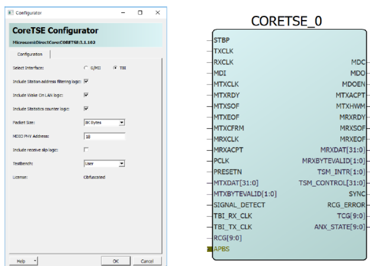
Figure 14 • CoreTSE Configuration in SGMII Mode
