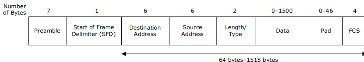
Figure 19 • Standard Ethernet Frame Format
