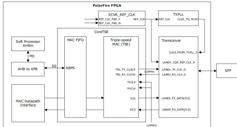
Figure 15 • SFP Connections for SGMII-Based Designs (Non-AMBA AHB)
