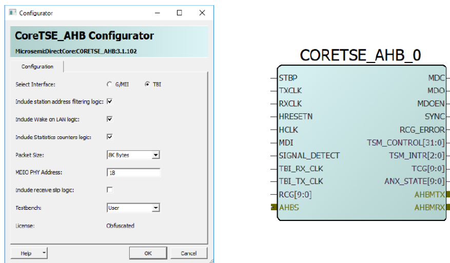
Figure 8 • CoreTSE_AHB Configuration in SGMII Mode
