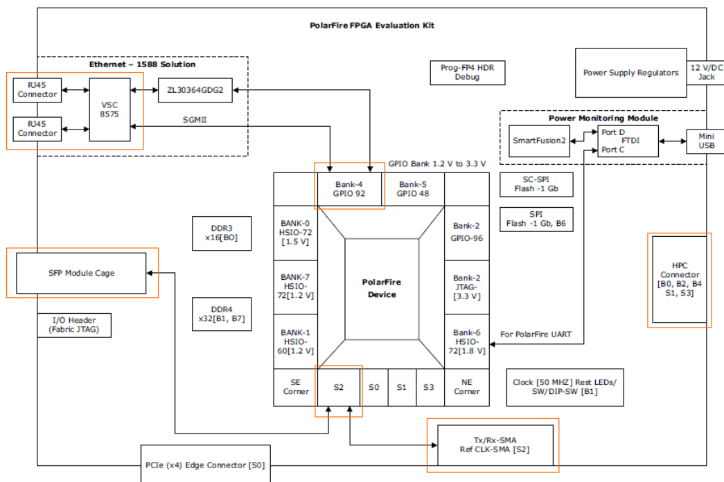
Figure 2 • PolarFire FPGA Evaluation Board Hardware Block Diagram
