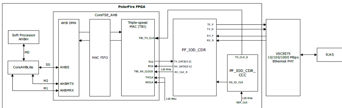
Figure 7 • RJ45 Connections for SGMII-Based Designs (AMBA AHB)
