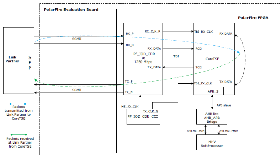
Figure 17 • SFP Connections for SGMII-Based Designs (for IOD-CDR)
