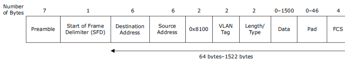
Figure 20 • Ethernet VLAN Frame Format
