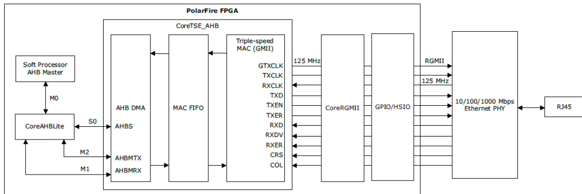
Figure 5 • RJ45 Connections for RGMII-Based Designs (AMBA AHB)
