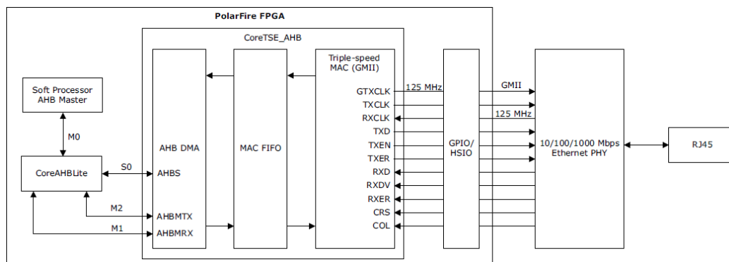
Figure 4 • RJ45 Connections for GMII-Based Designs (AMBA AHB)
