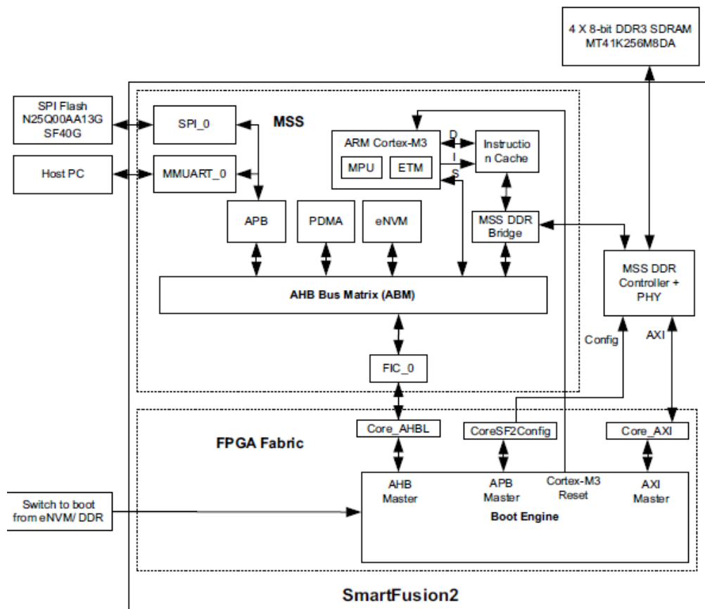
Figure 6 • Design Flow for Hardware Boot Engine Method
