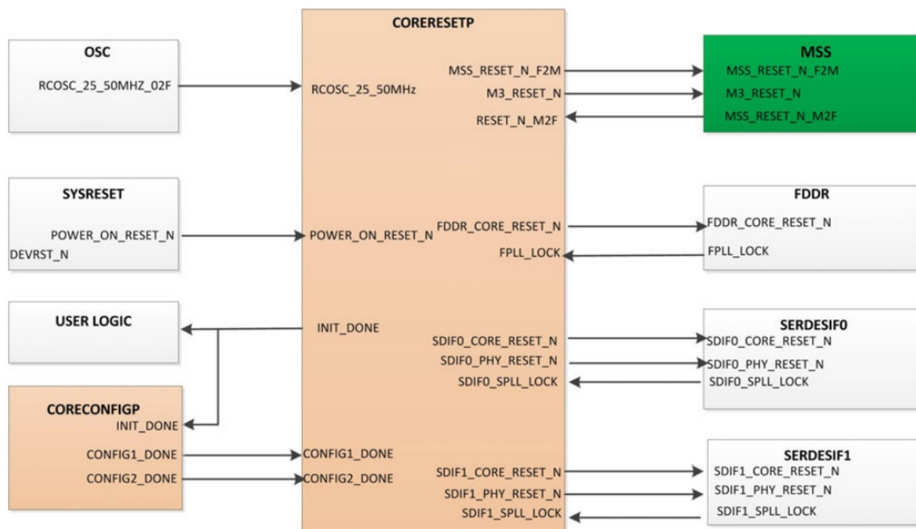
Figure 3-8 • Core SF2Reset Sub-System Connectivity
