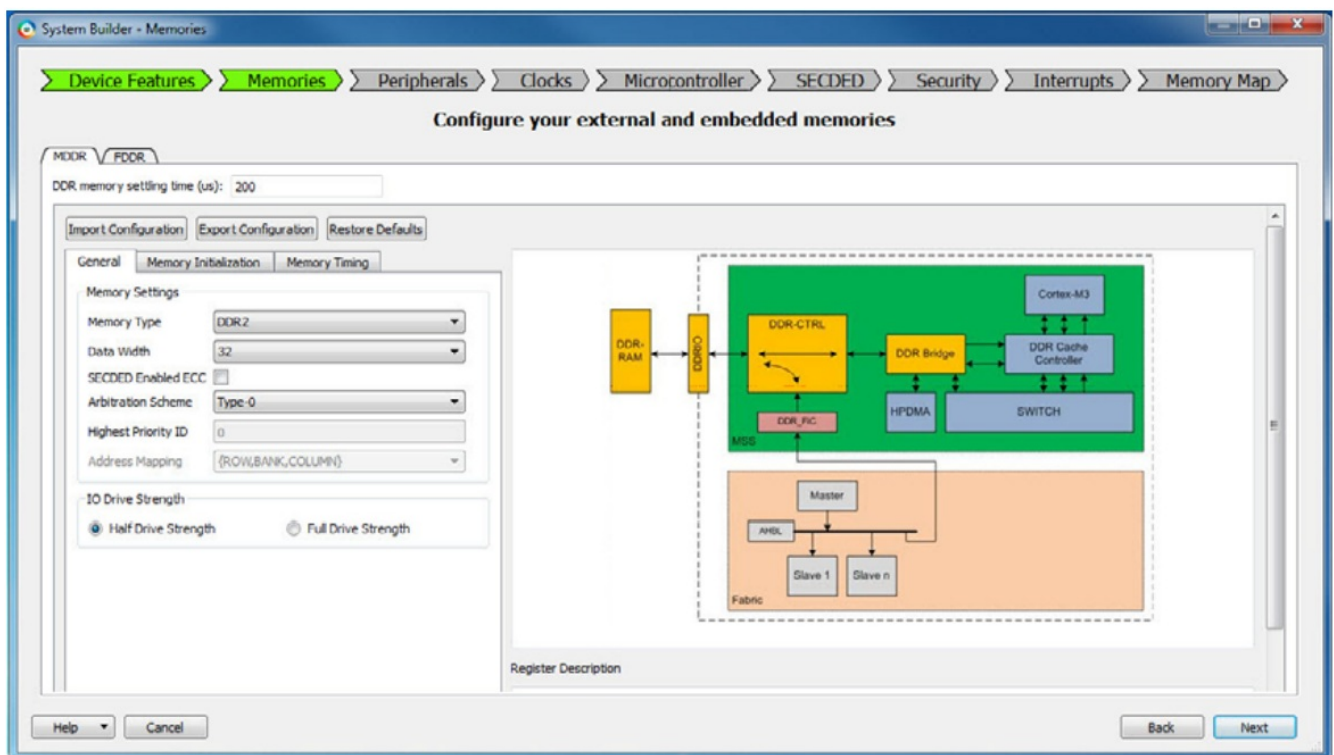
Figure 2-2 • MSS External Memory
