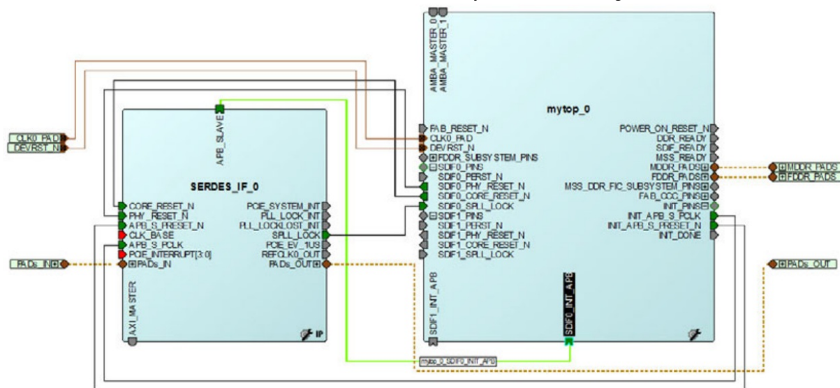
Figure 2-7 • SERDESIF Peripheral Initialization Connectivity
