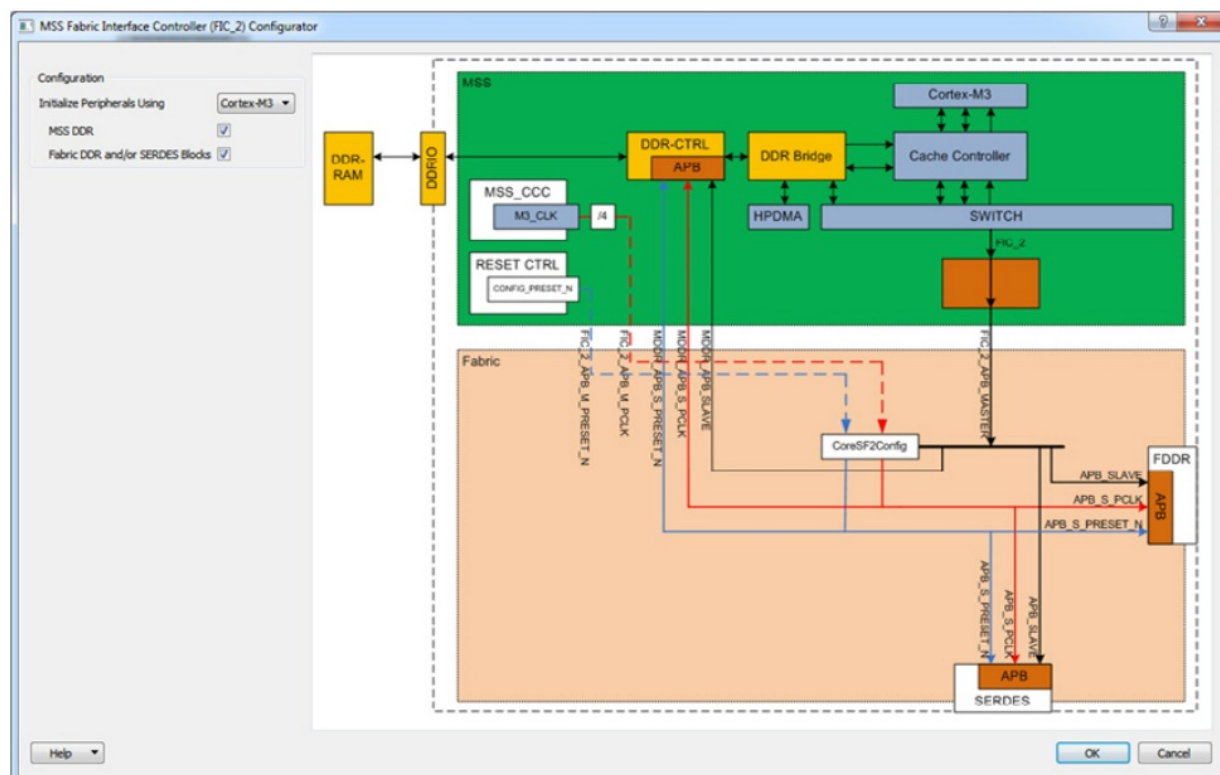
Figure 3-2 • MSS FIC_2 Configurator
