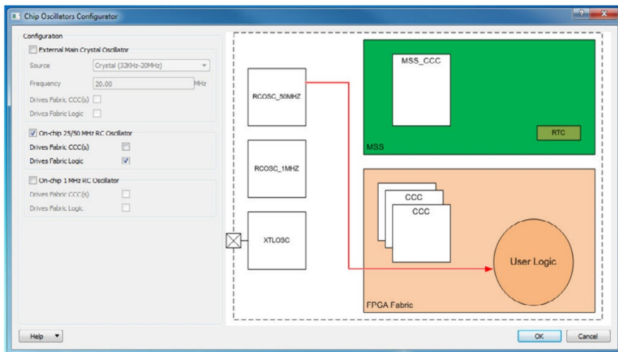
Figure 3-5 • Chip Oscillators Configurator
