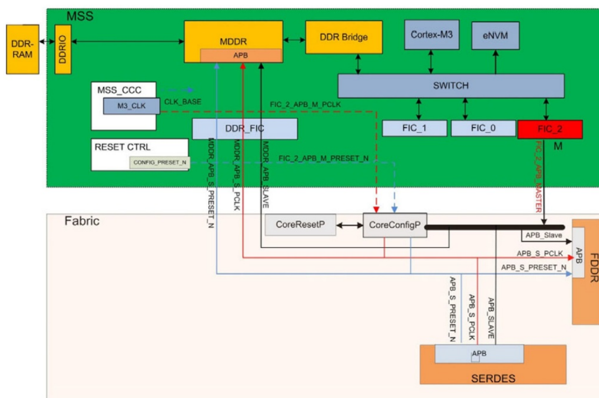
Figure 3-7 • FIC_2 APB3 Sub-System Connectivity
