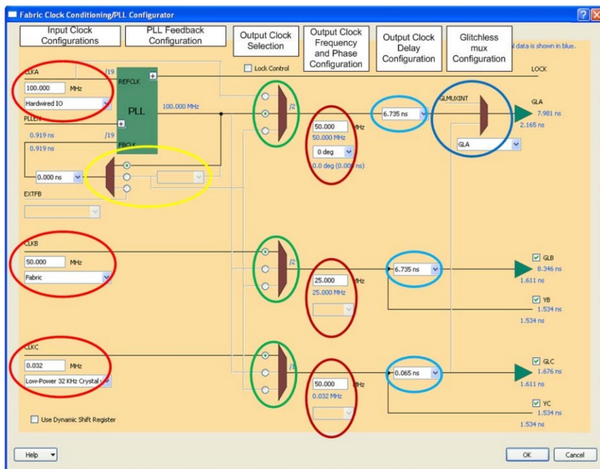
Figure 1-1 • FAB_CCC Configuration Options
