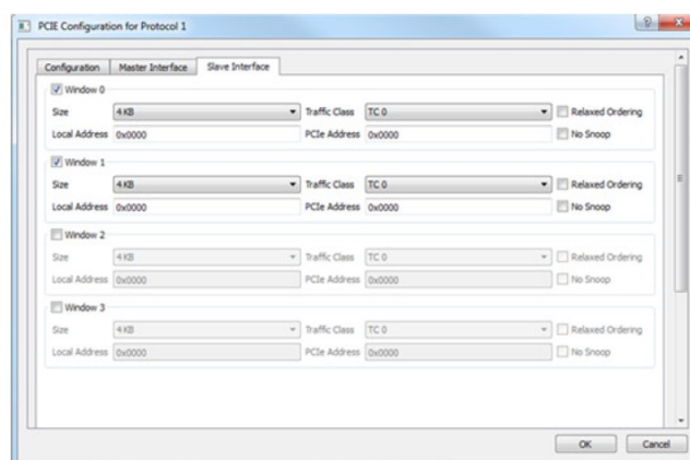
Figure 1-4 • PCIe Configuration - Slave Interface Tab
