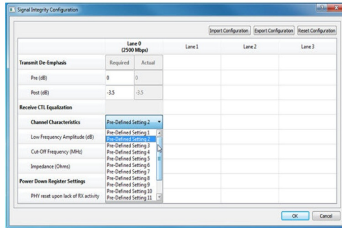
Figure 1-7 • Signal Integrity Configuration Dialog Box
