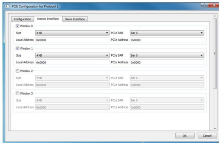
Figure 1-3 • PCIe Configuration - Master Interface Tab
