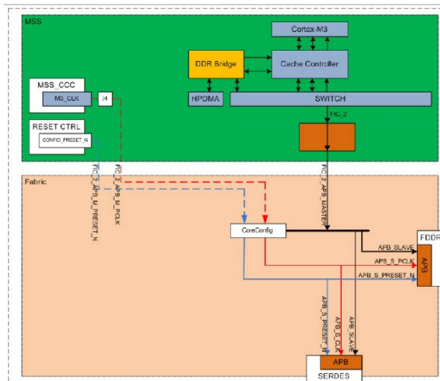
Figure 1-9 • FIC_2 Configurator Overview
