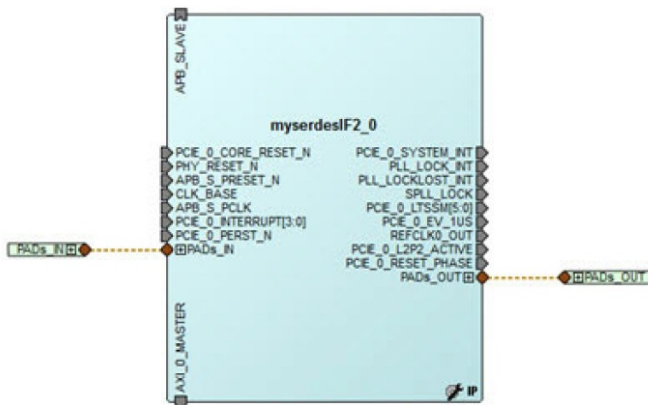
Figure 1 • SERDES IF2 Block Instantiation on the SmartDesign Canvas
