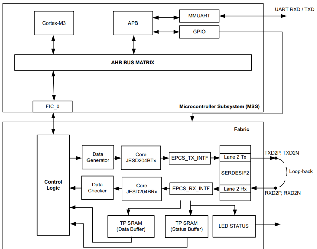
Figure 2 • Hardware Implementation Block Diagram
