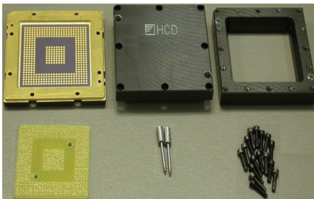
Figure 1 • CCGA to FBGA Adapter Socket Components
