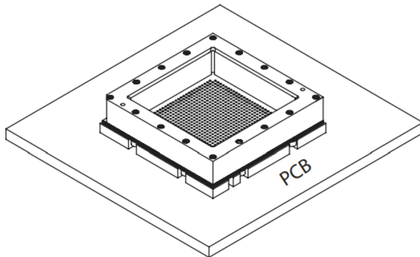
Figure 6 • Adapter Reflowed to the PCB
