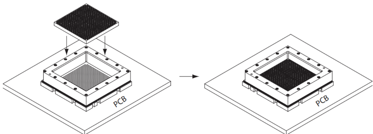
Figure 7 • Socket Interposer Placement in the Adapter Assembly
