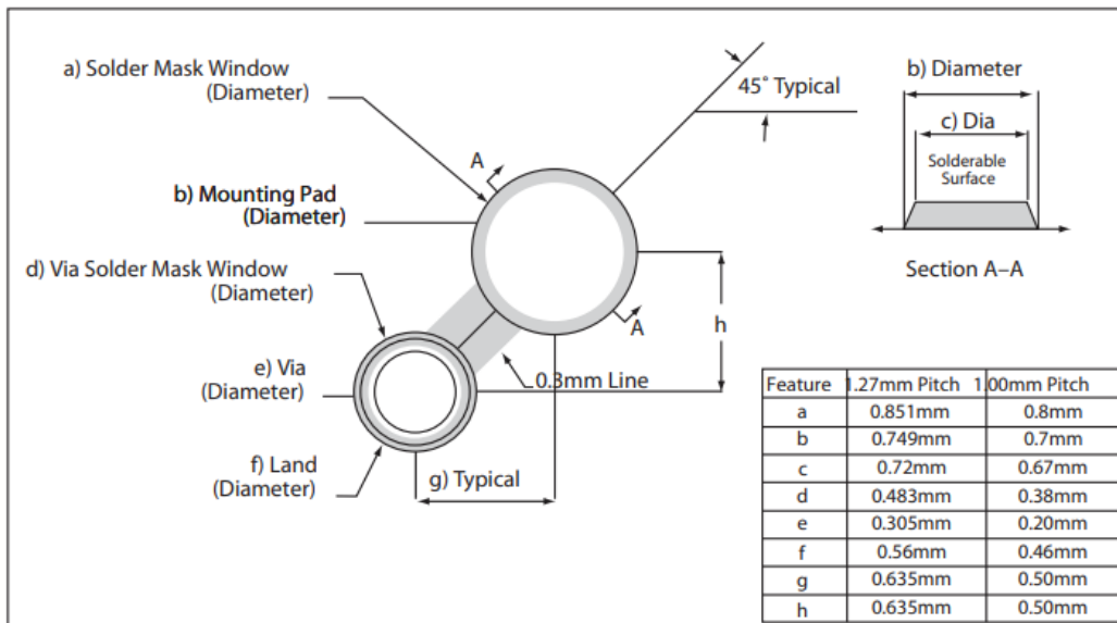
Figure 10 • PCB Pad Layout Specifications
