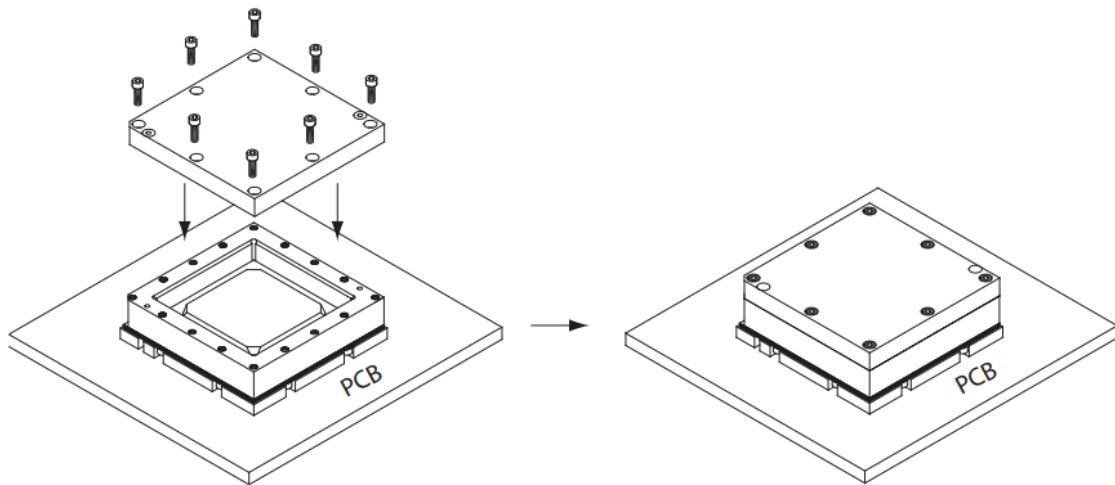
Figure 9 • View of the Socket Lid and Screw Placement
