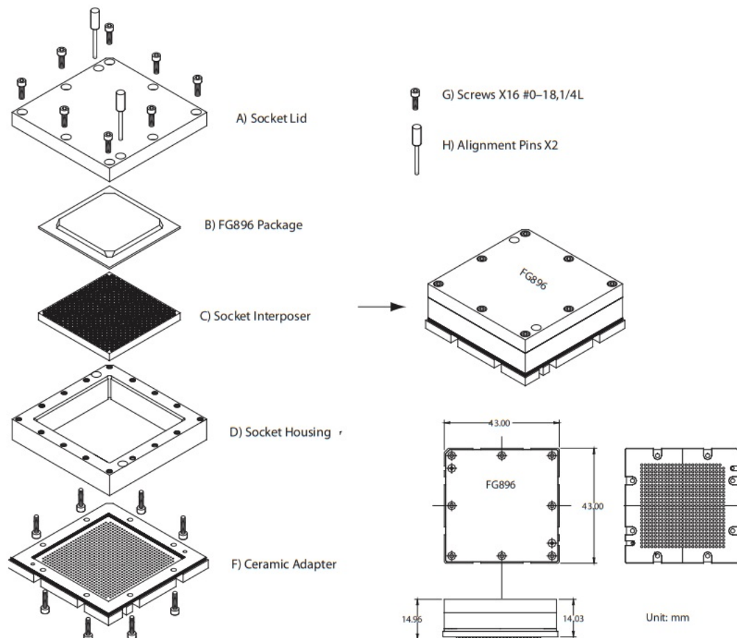
Figure 12 • CG624 to FG896 Adapter Socket Outline Drawing
