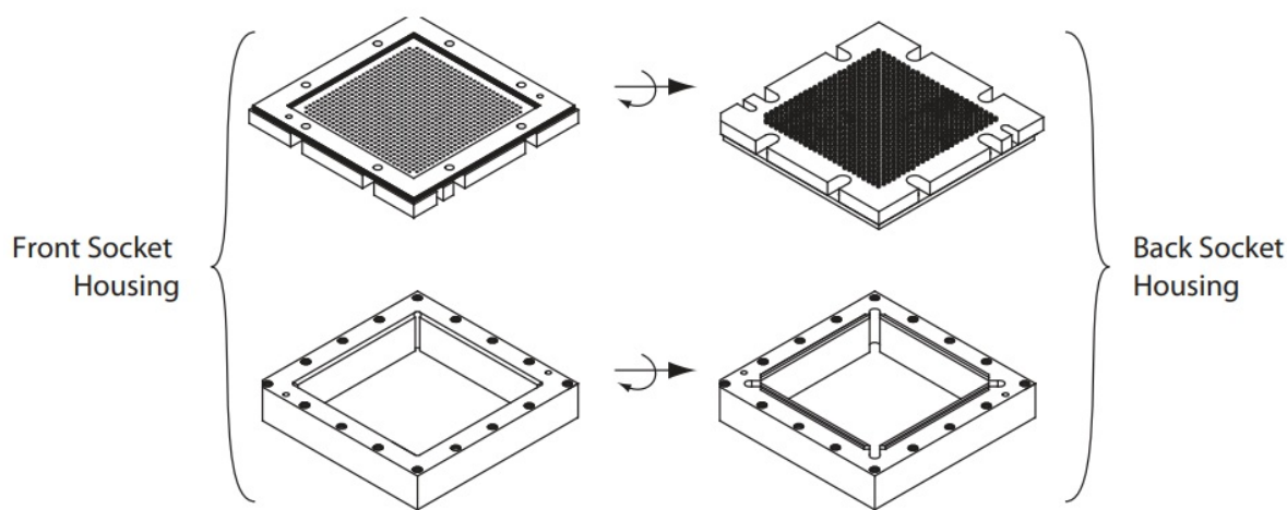
Figure 3 • View of Ceramic Adapter (Top) and Socket Housing (Bottom) Turned Over
