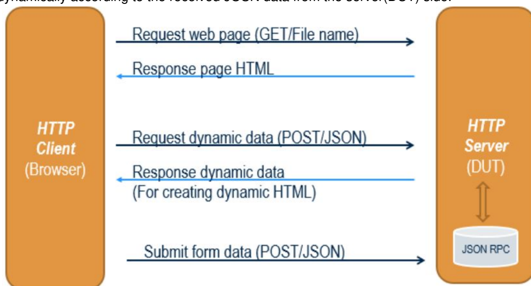
Figure 1. The access flow between client and server
