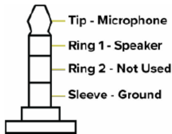
Figure 4: TRRS Connector
