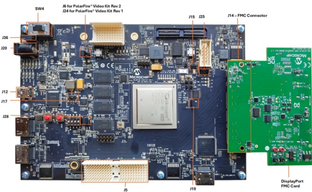
Figure 3-1. Setting up the Hardware
