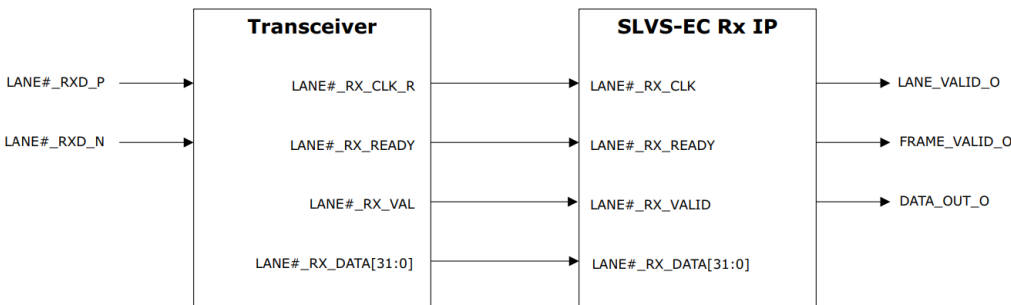
Figure 1 • SLVS-EC IP Block Diagram
