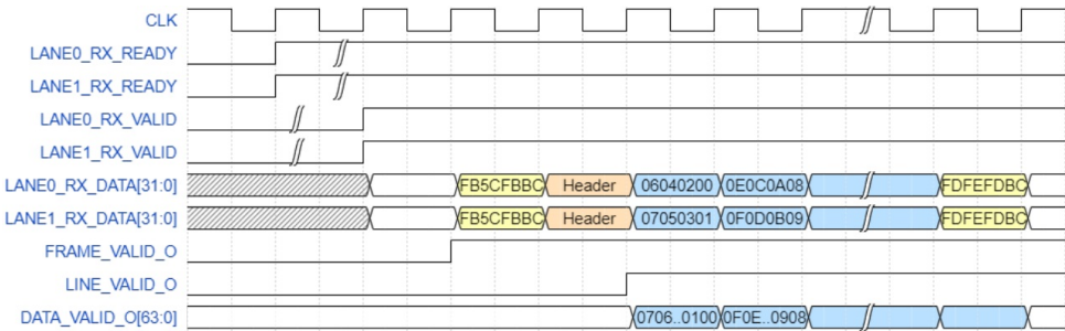
Figure 9 • SLVS-EC IP Timing Diagram
