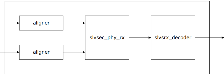
Figure 6 • Internal Blocks of the SLVS-EC RX IP
