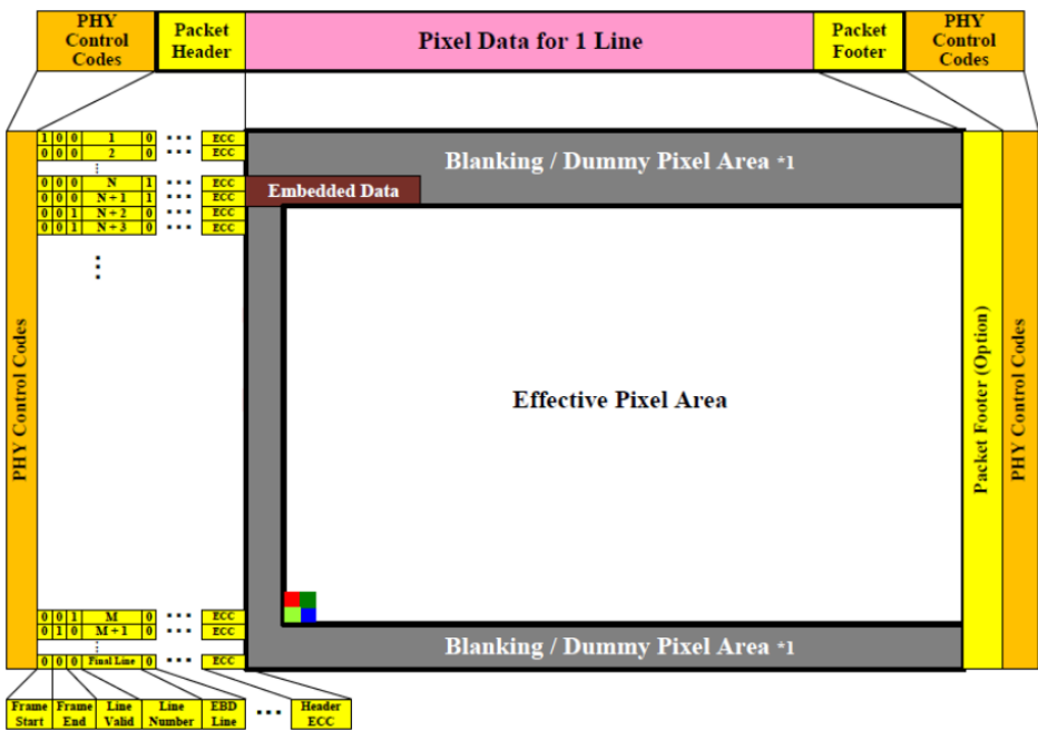
Figure 5 • SLVS-EC Frame Format Structure
