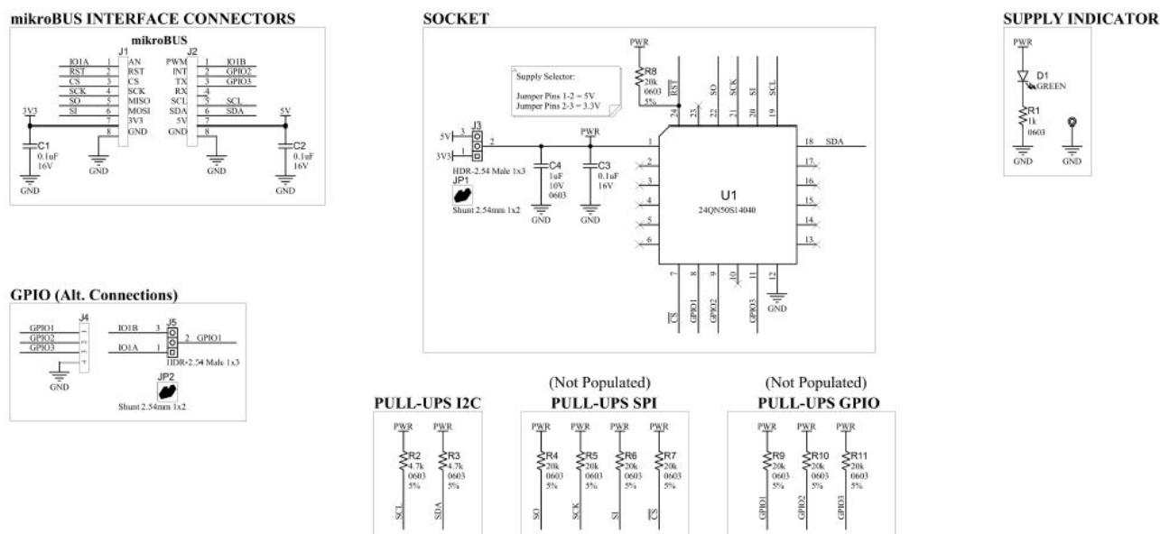
Figure 1-1. TA100 24-Pad VQFN Socket Board Schematic
