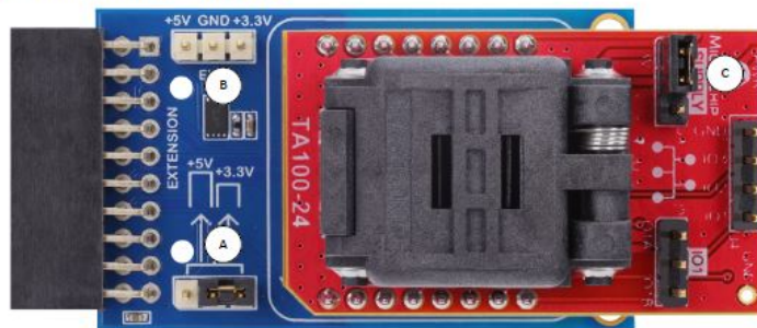
Figure 2-2. ATMBUSAdapter Plus EV39Y17A
