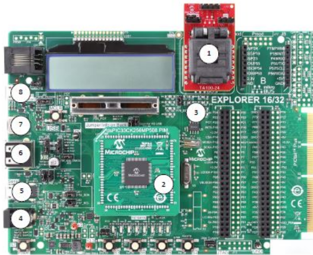
Figure 2-3. Connections to a Microchip Explorer 16/32 Development Board
