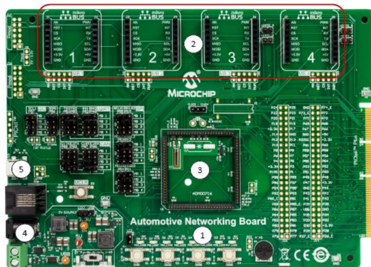
Figure 2-4. Connections to the Automotive Networking Development Board
