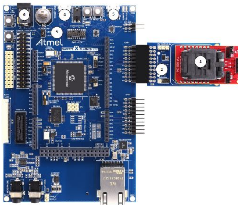
Figure 2-1. Connections to an Xplained Pro Development Platform
