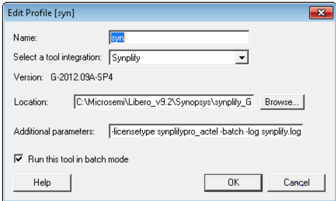
Figure 2-2. Example to Invoke Synplify from Within Libero
