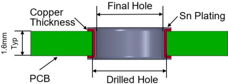
Figure 1-1. PCB Construction
