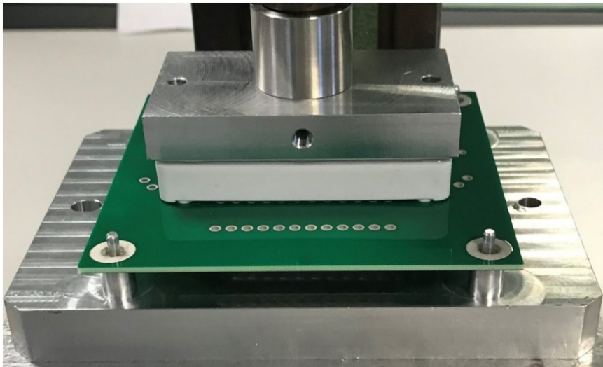
Figure 3-3. PressFIT Pins into the PCB
