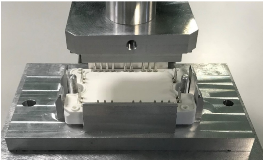
Figure 6-3. Module Removed
