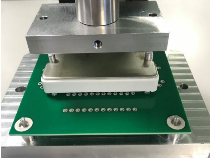
Figure 3-2. PCB with Module before the Insertion
