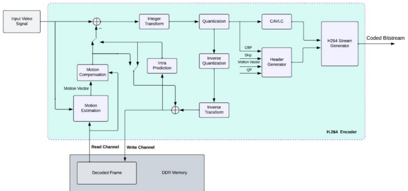
Figure 1-1. H.264 Encoder – Modules
