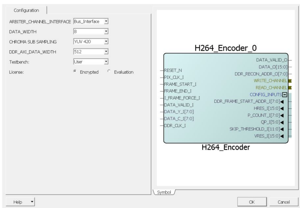
Figure 7-1. H.264 Encoder Configurator
