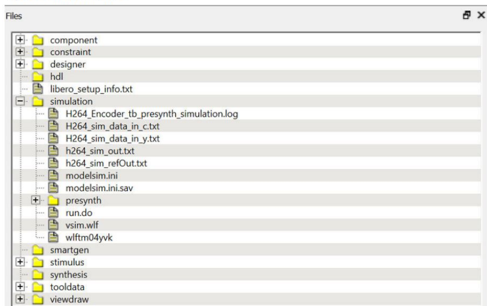
Figure 5-5. Imported Files
