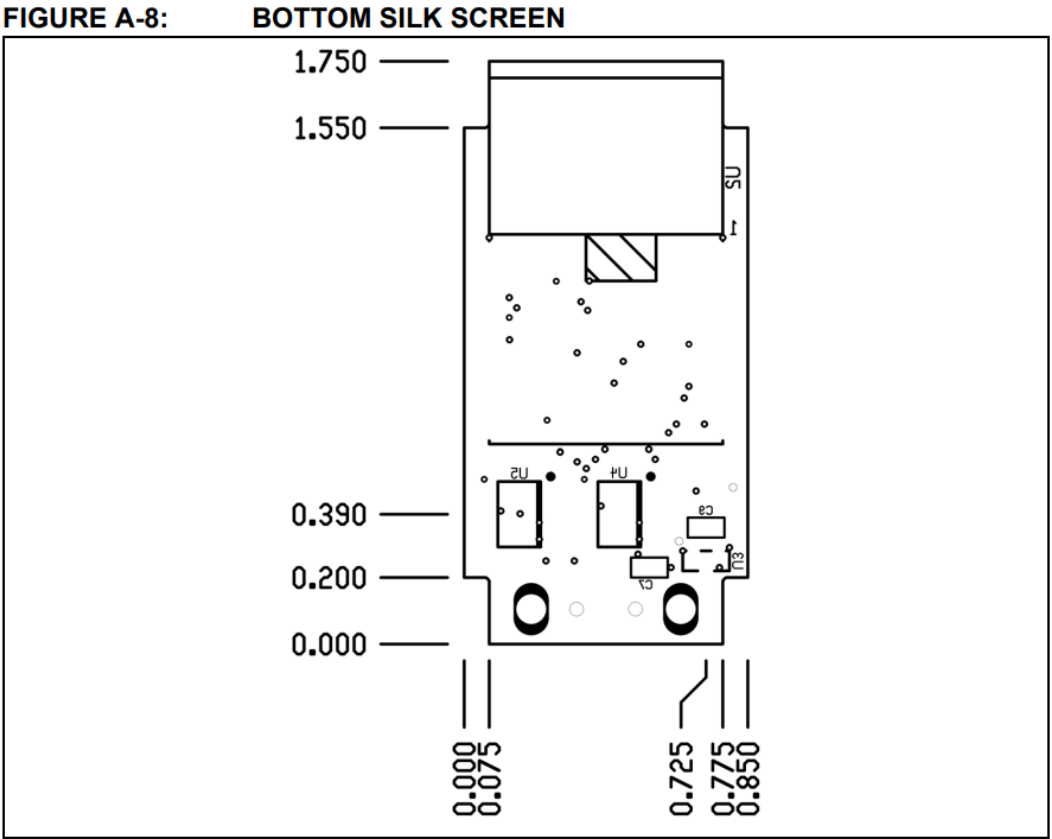
Figure A-8 illustrates the ZENA Wireless Adapter bottom silk screen.
