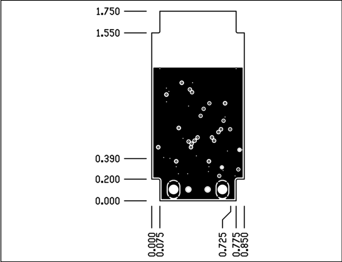
FIGURE A-5: LAYER 2 — GROUND PLANE
