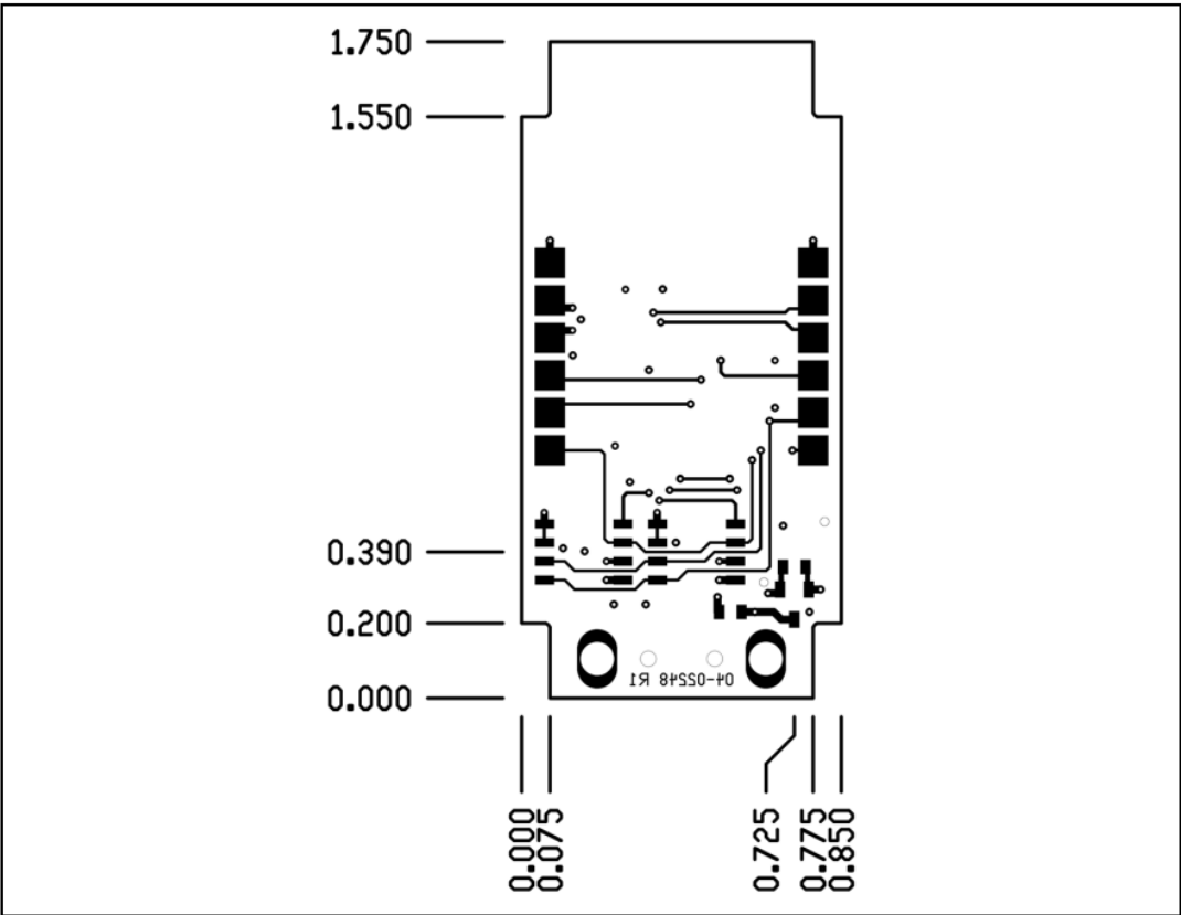
FIGURE A-7: LAYER 4 — BOTTOM COPPER
