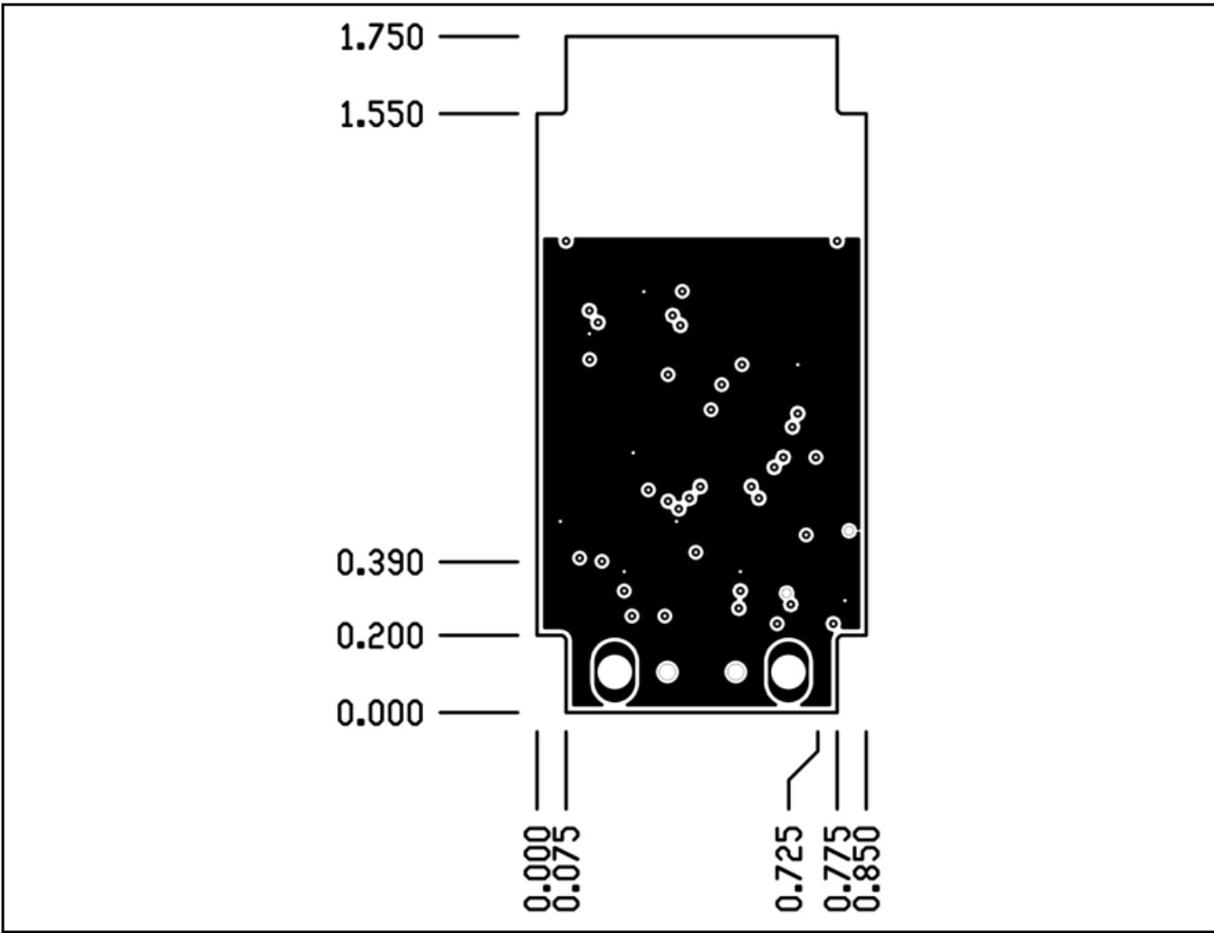
FIGURE A-6: LAYER 3 — POWER PLANE
