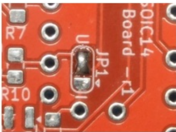
Solder jumper selecting UPDI programming option
